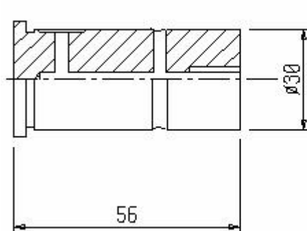
G9/030P Bolzen 305-08-1410
