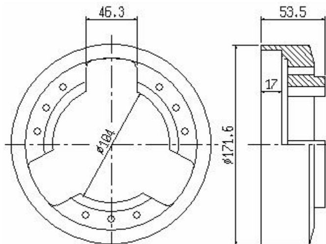
G9/003 Spannfinger AS82 327-10-2130/002 100630
