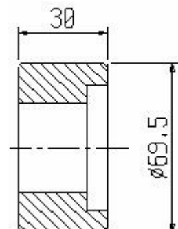
G9/035R Rolle
