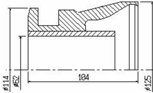
S4/001 mufa zacisku SD32 376+329
