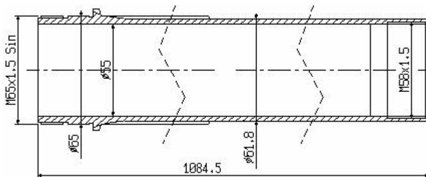
S5/012 Rura posuwu
