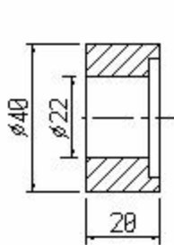
S5/033R Rolka
